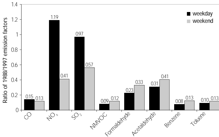
FIGURE 4.26 Changes in road tunnel emission factors between 1988 and 1997 in the Tauertunnel, Austria
