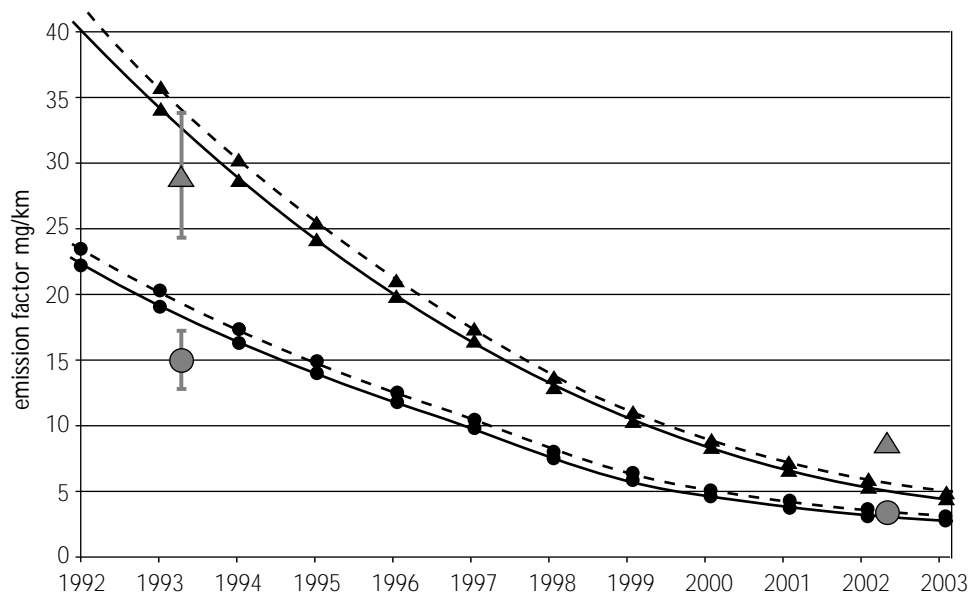
FIGURE 4.22 Modelled (lines) and measured (points) emission factors for benzene (lower lines) and toluene (upper lines) in the Gubristtunnel, Zurich
