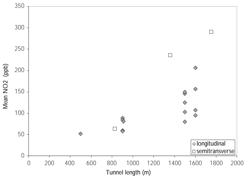
FIGURE 4.10 Relationship between mean NO 2 and tunnel length for a range of urban tunnels as a function of ventilation type
