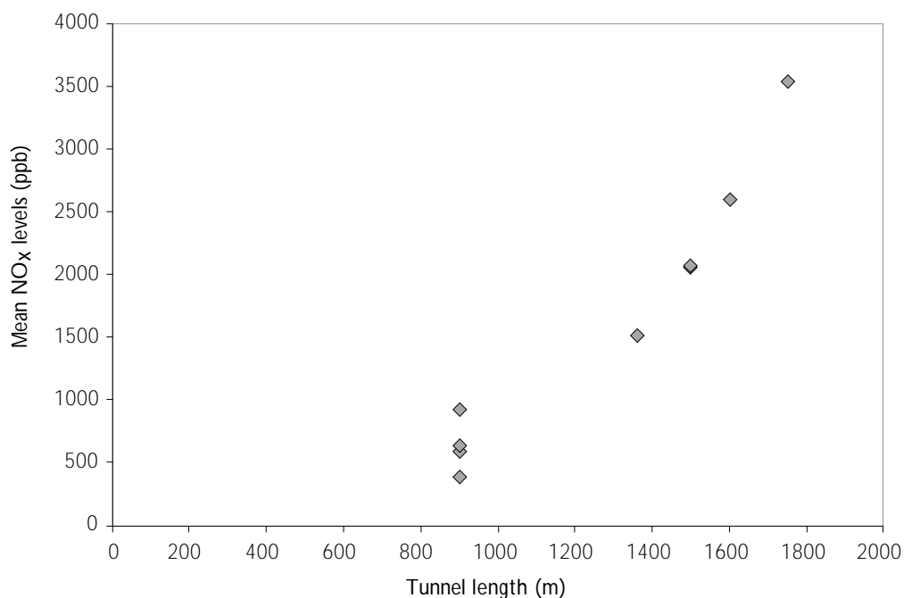
FIGURE 4.8 Relationship between mean \text{NO}_x in a range of tunnels as a function of their length
