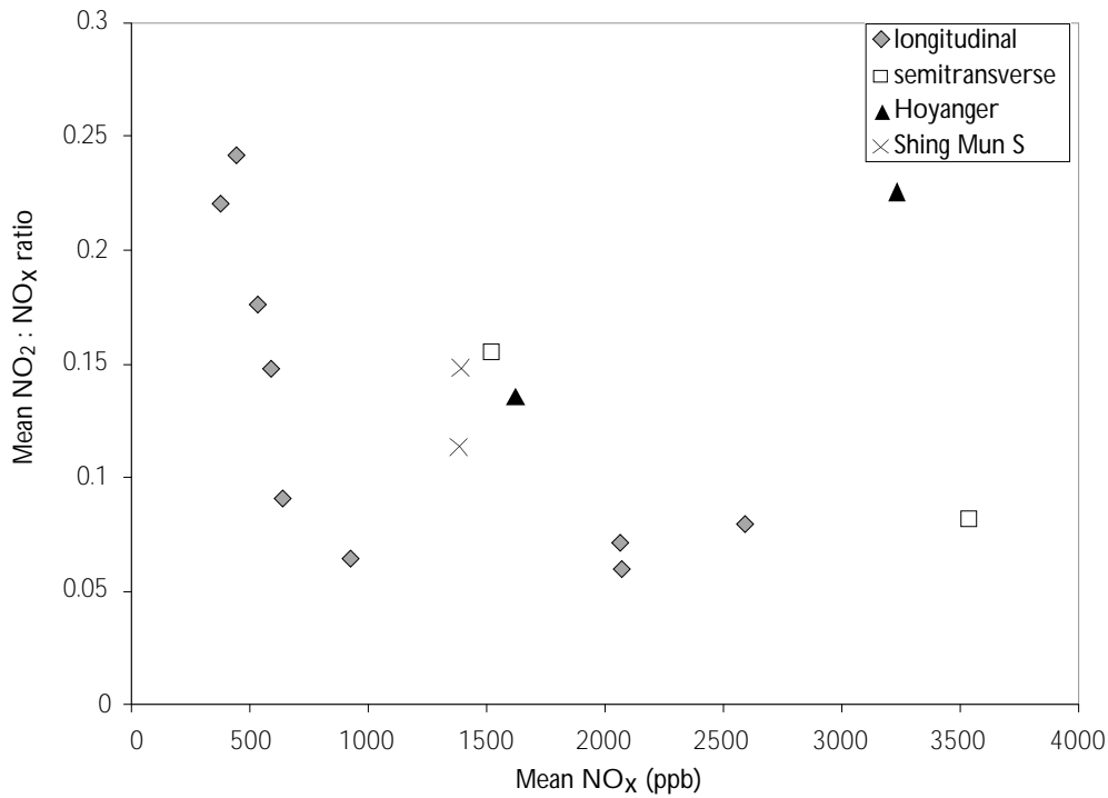
FIGURE 4.9 Dependence of the ratio of mean NO 2 to mean NO x on NO x for a range of road tunnels as a function of ventilation type
